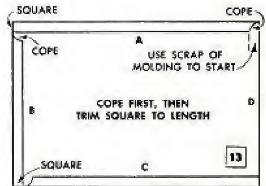
Some workmen prefer to undercut the cope with a rotary file, or burr, driven by means of a hand grinder
